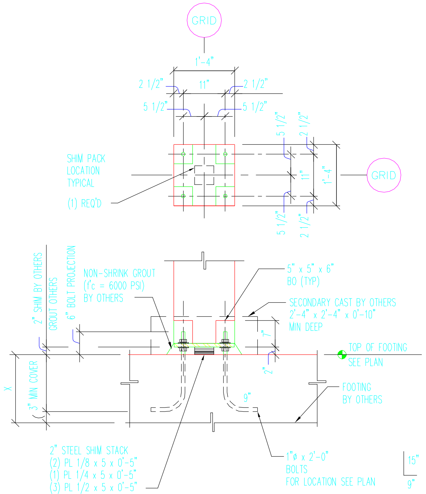
1'-4" x 1'-4" COLUMN FOUNDATION CONNECTION STANDARD COLUMN DETAIL
